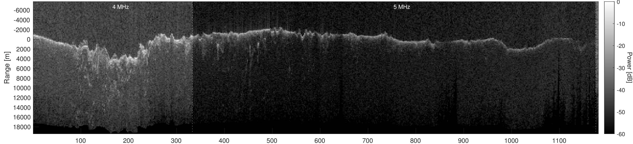
Orbit 12440, Optimized, Window, Depth-Corrected, Channel 2
