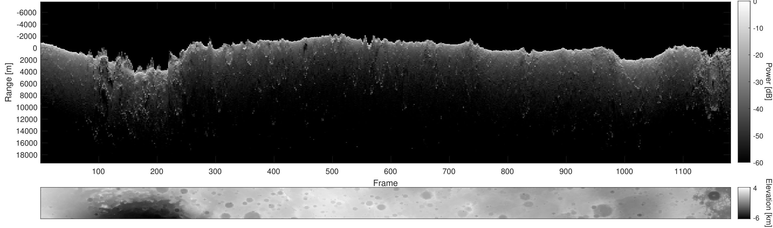
Orbit 12440, Depth-Corrected Cluttergram
