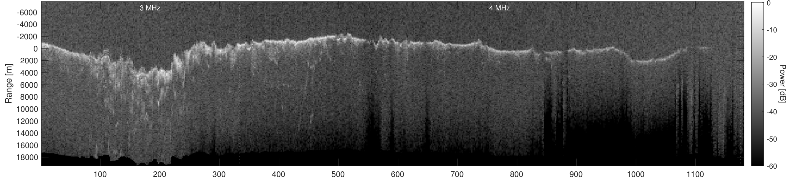
Orbit 12440, Depth-Corrected Cluttergram
