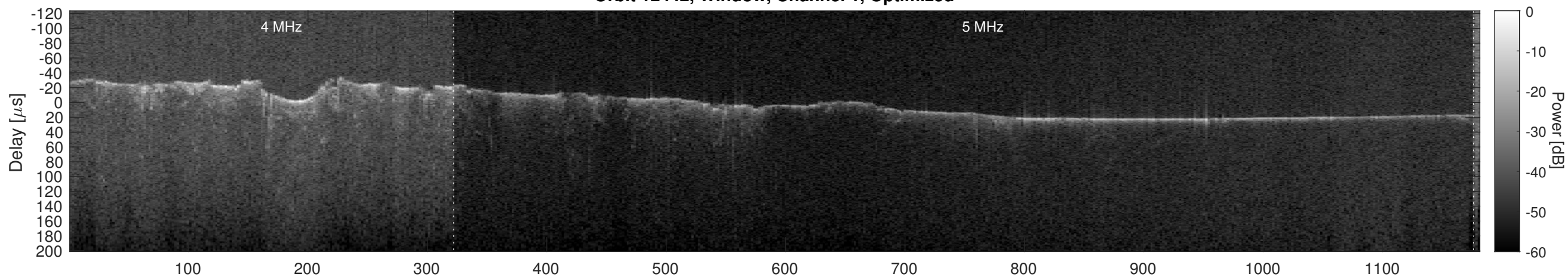
Orbit 12442, Cluttergram
