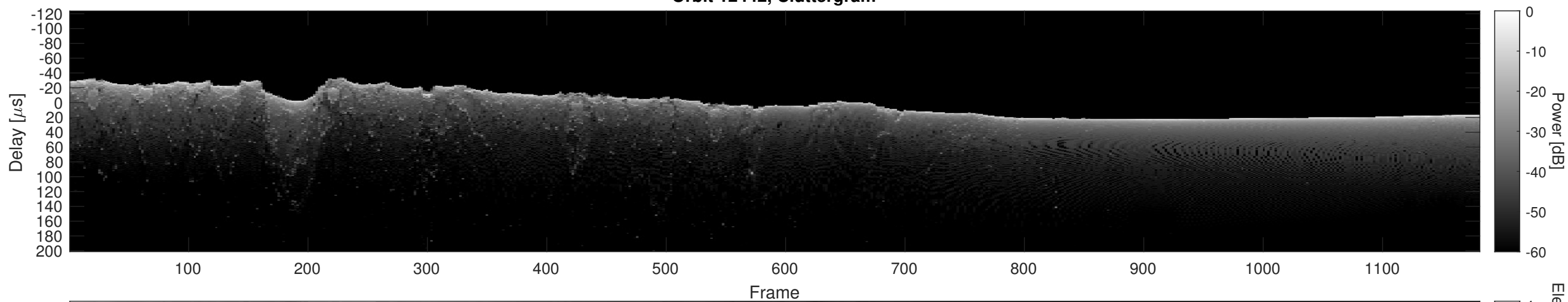
Orbit 12442, Cluttergram
