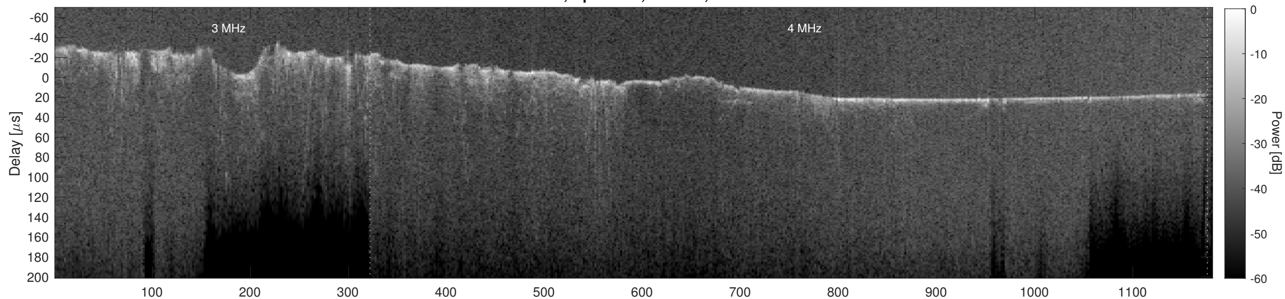
Orbit 12442, Cluttergram
