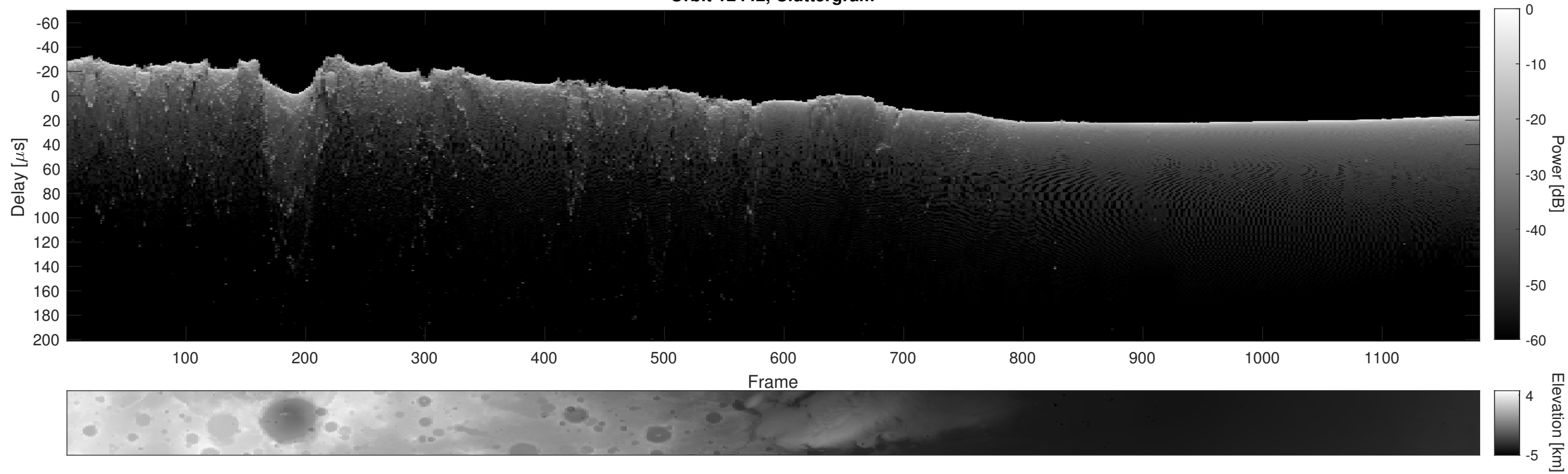
Orbit 12442, Cluttergram
