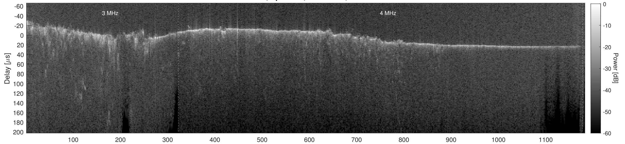
Orbit 12443, Cluttergram
