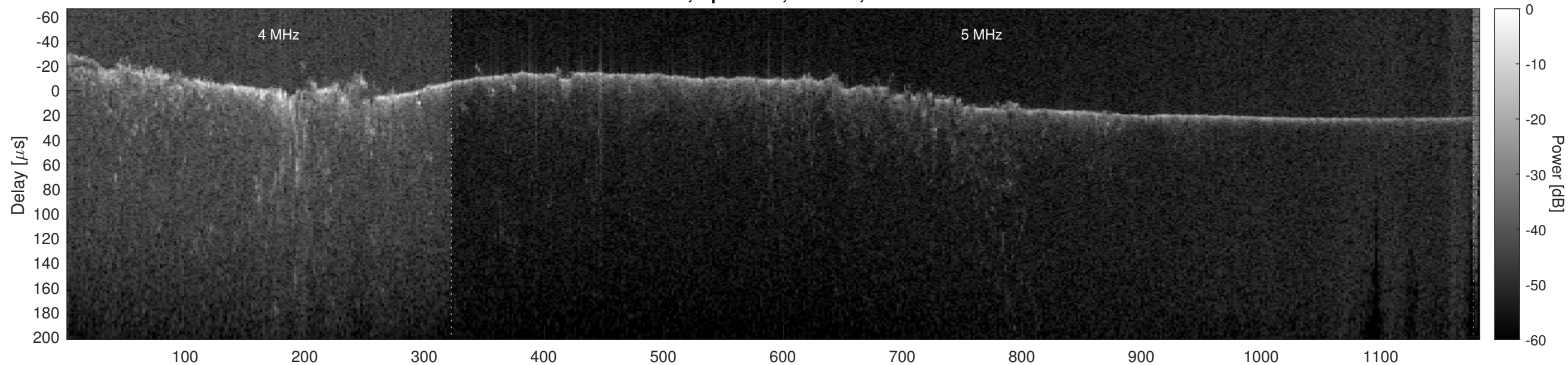
Orbit 12443, Optimized, Window, Channel 2
