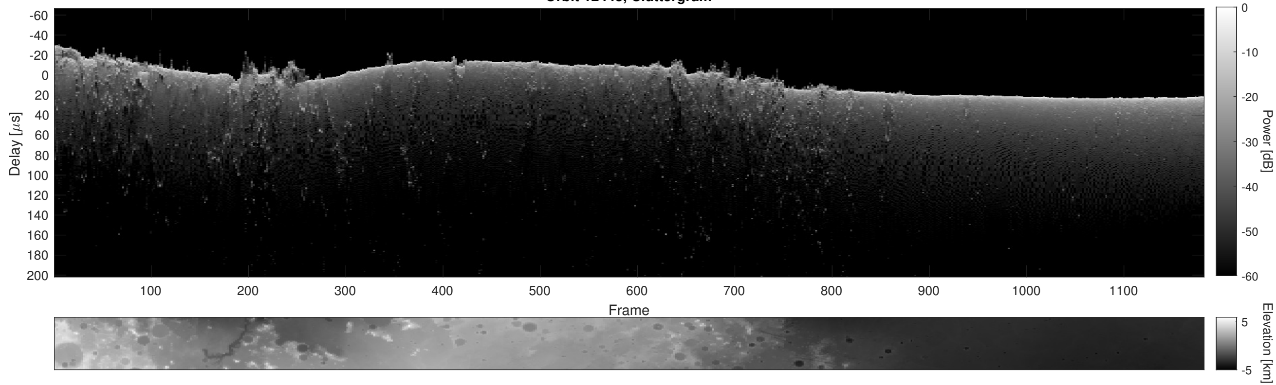
Orbit 12443, Cluttergram
