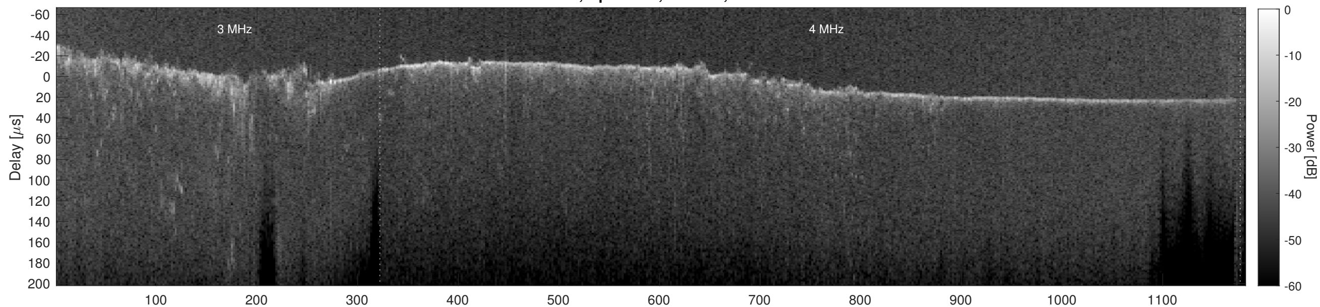
Orbit 12443, Cluttergram
