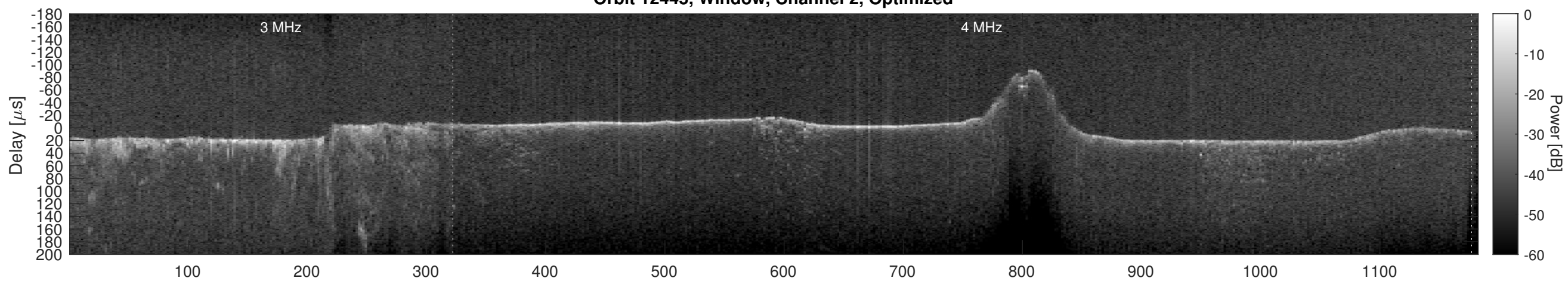
Orbit 12445, Cluttergram
