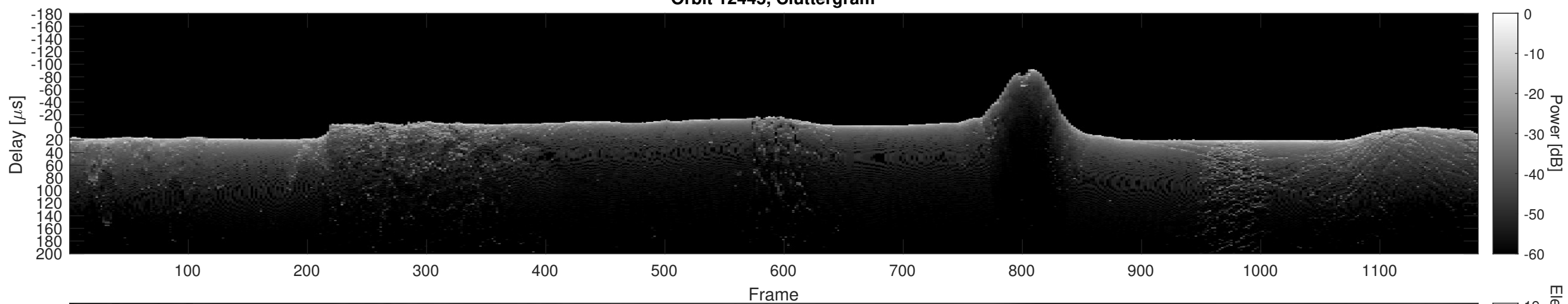
Orbit 12445, Cluttergram
