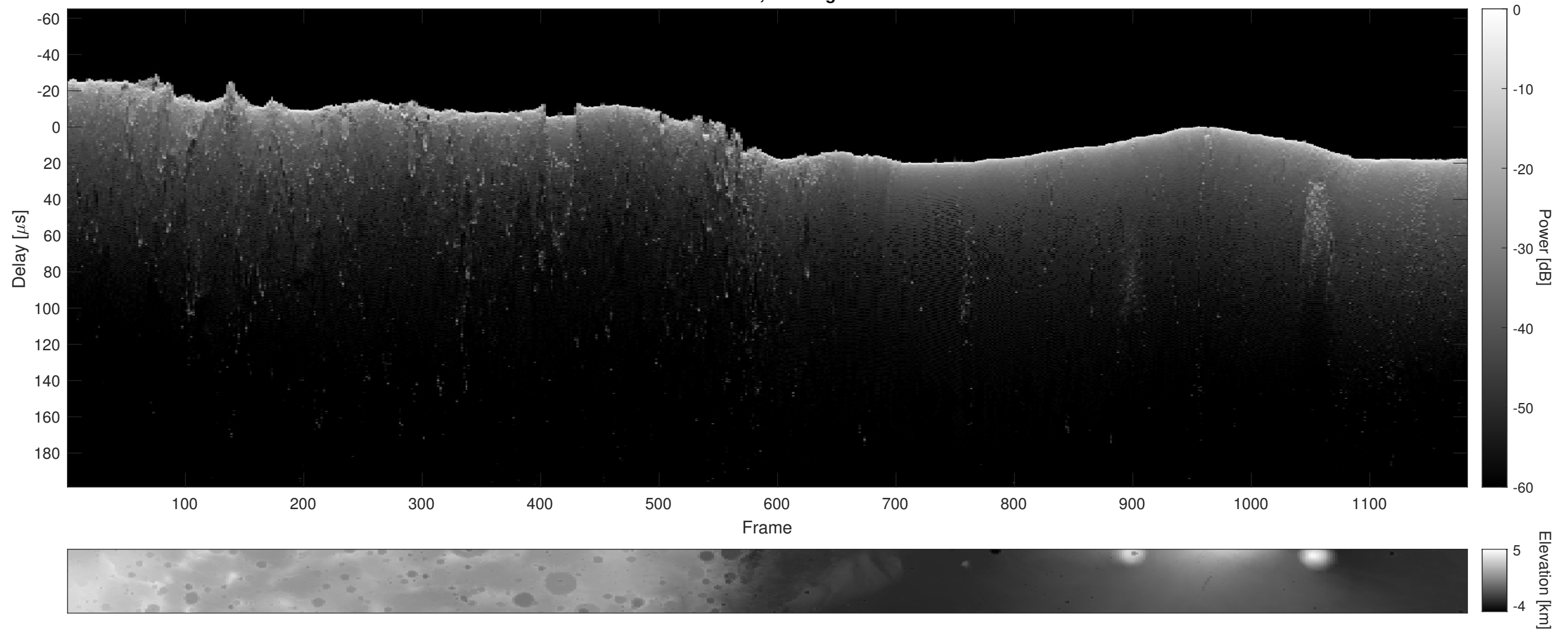
Orbit 12446, Cluttergram
