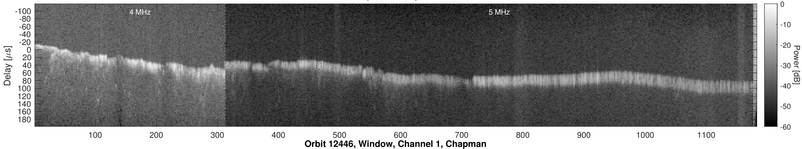
Orbit 12446, Channel 1, Uncorrected
