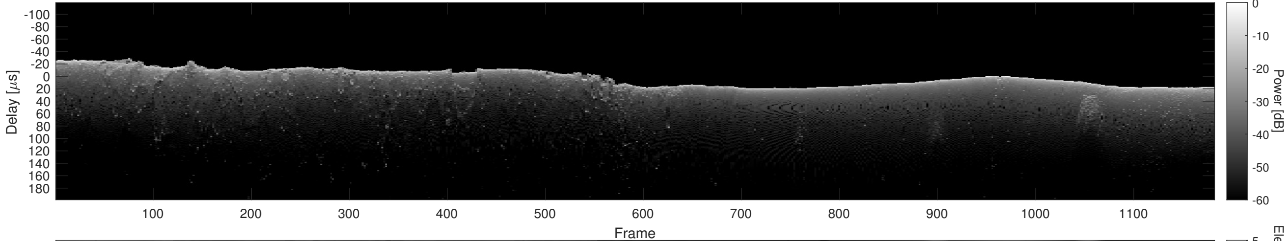
Orbit 12446, Cluttergram
