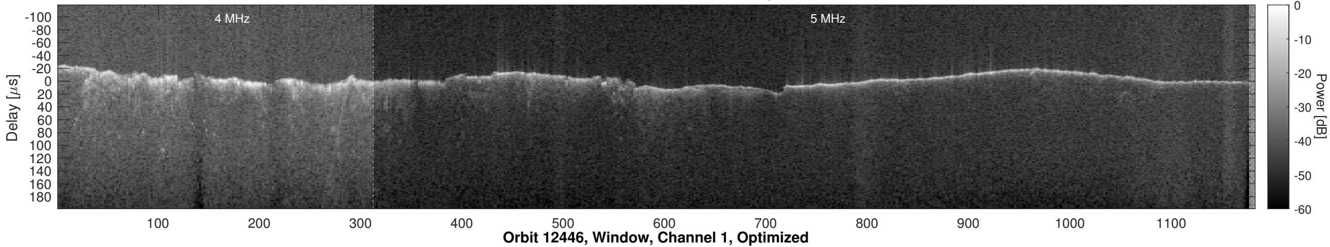
Orbit 12446, Window, Channel 1, Chapman
