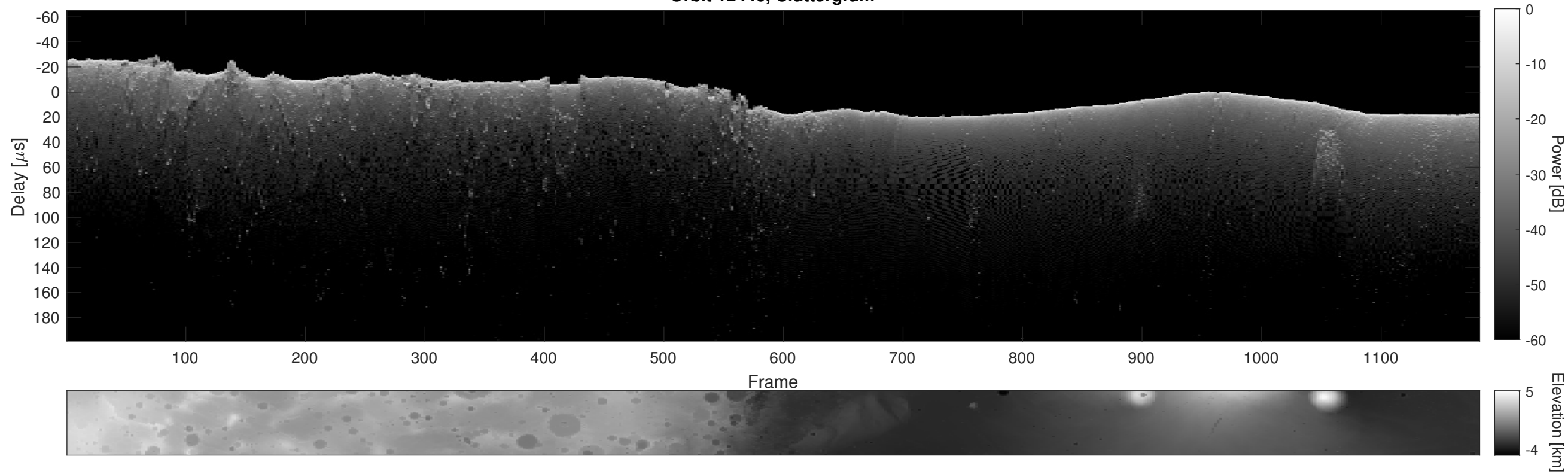
Orbit 12446, Cluttergram
