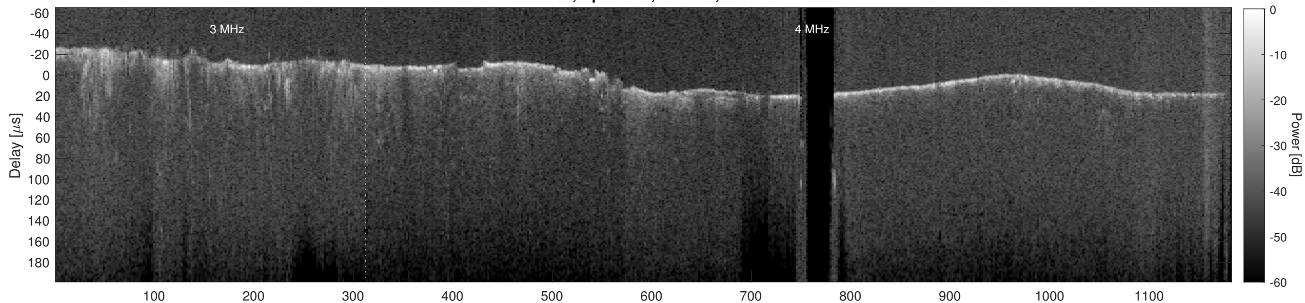
Orbit 12446, Cluttergram
