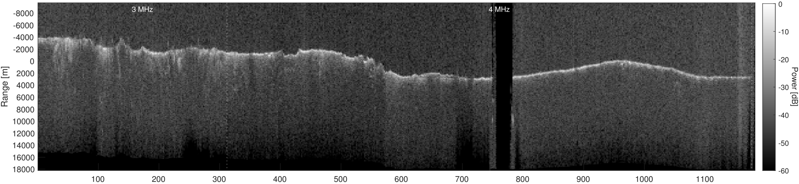
Orbit 12446, Depth-Corrected Cluttergram
