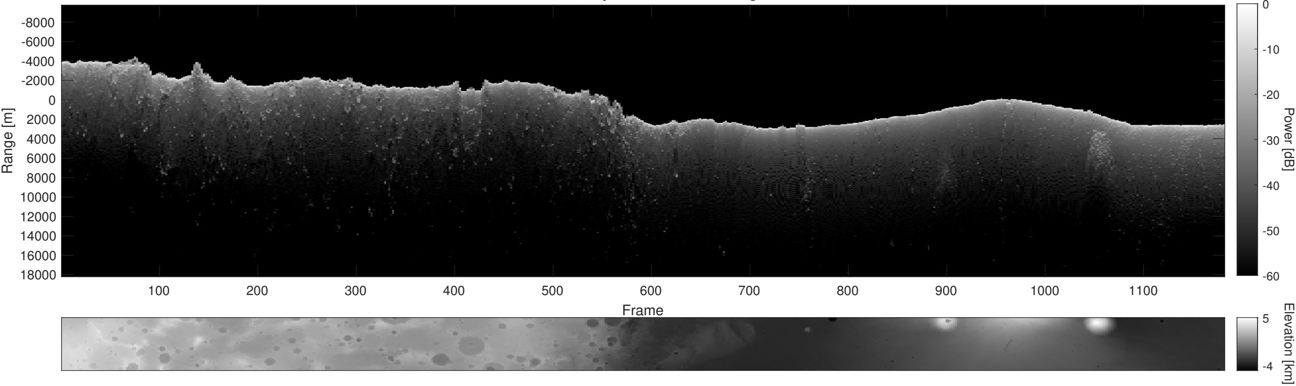
Orbit 12446, Depth-Corrected Cluttergram
