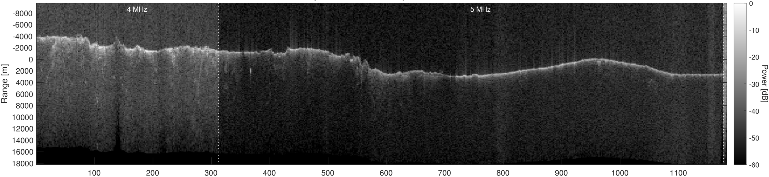
Orbit 12446, Optimized, Window, Depth-Corrected, Channel 2
