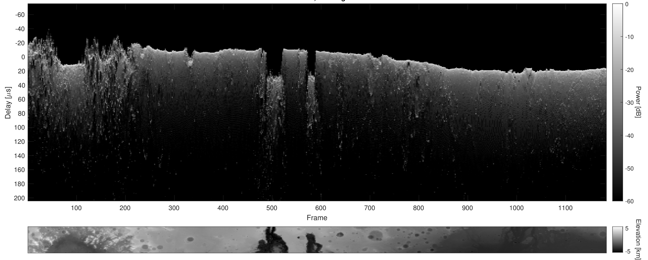
Orbit 12448, Cluttergram
