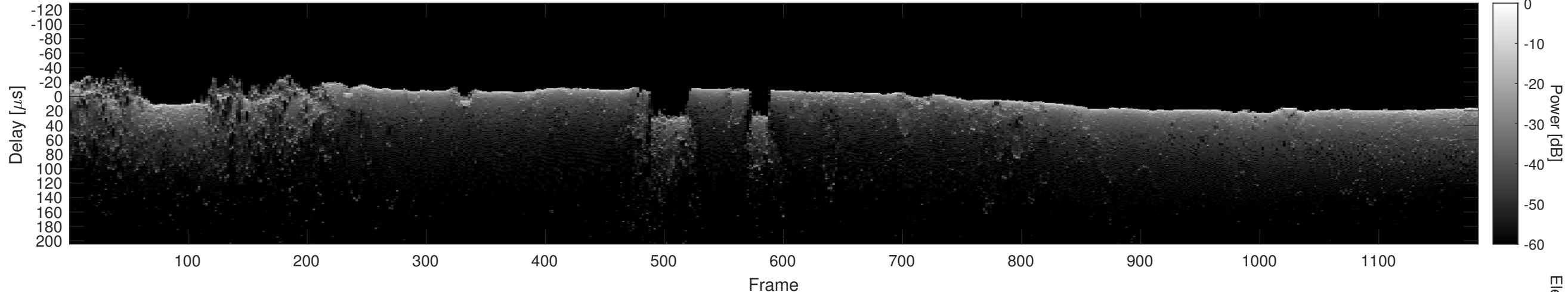
Orbit 12448, Cluttergram
