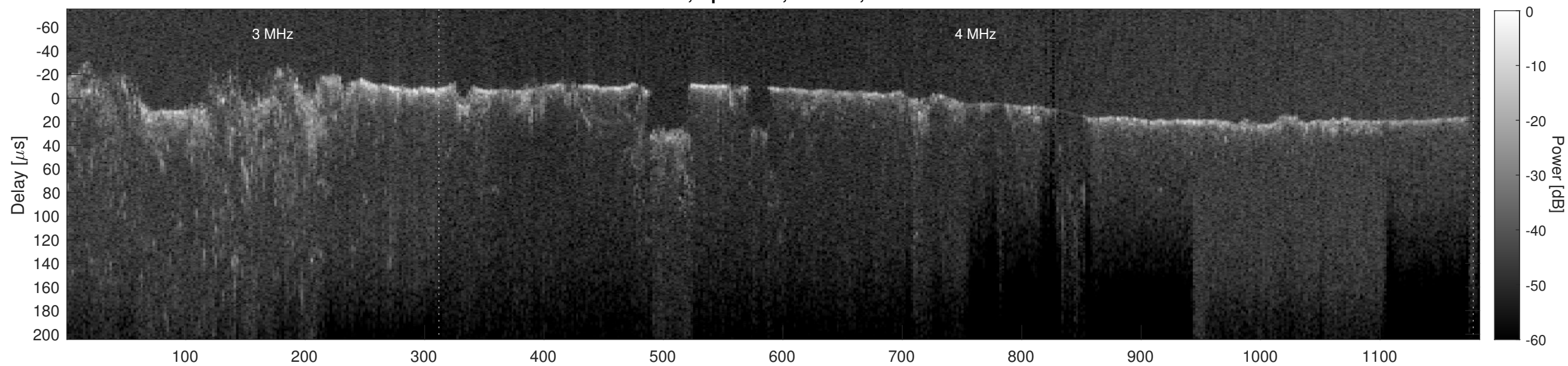
Orbit 12448, Cluttergram
