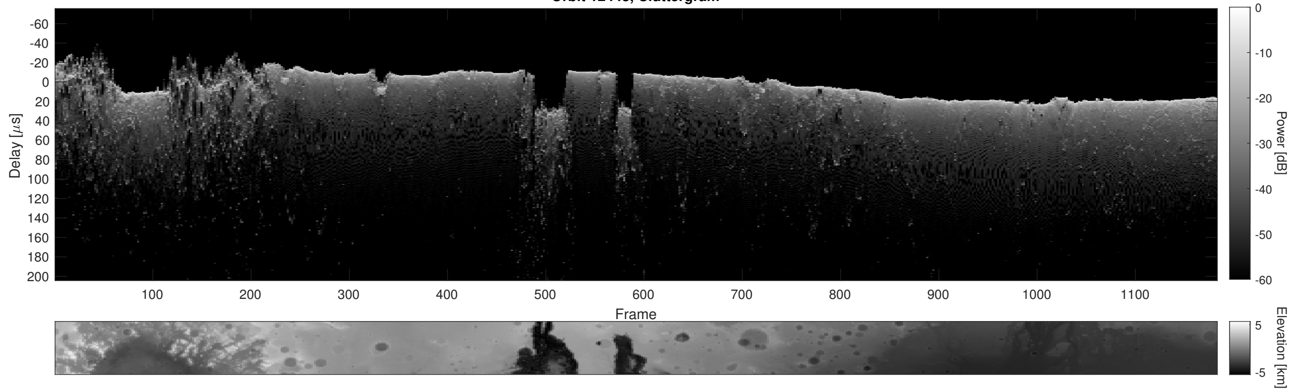
Orbit 12448, Cluttergram
