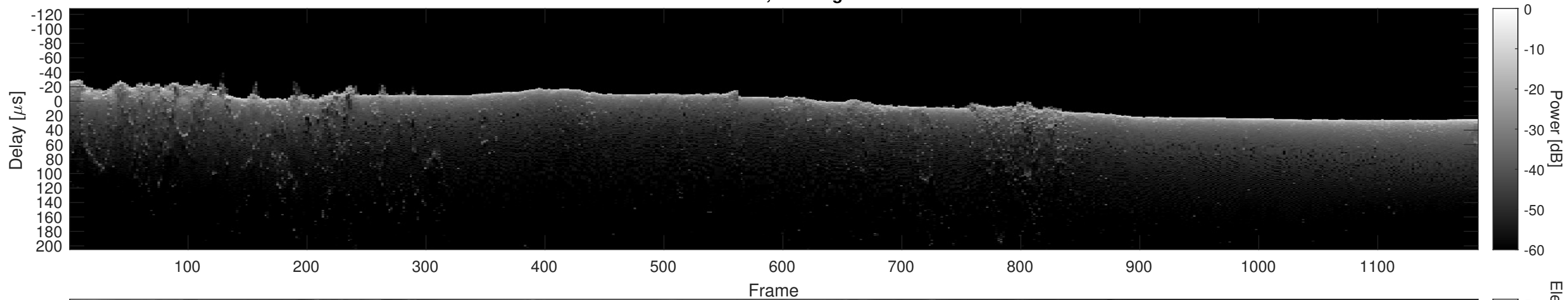
Orbit 12450, Cluttergram
