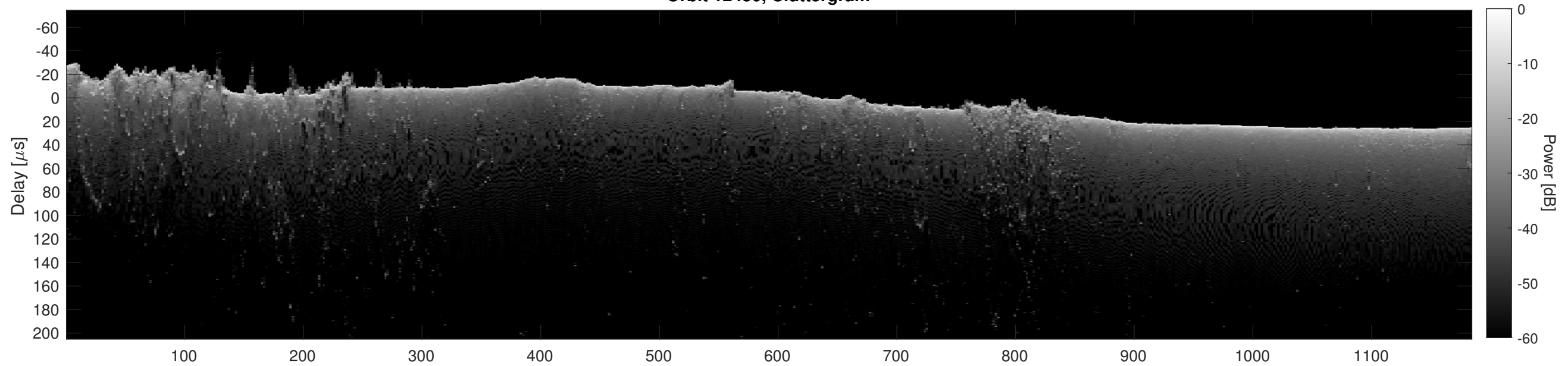
Orbit 12450, Cluttergram
