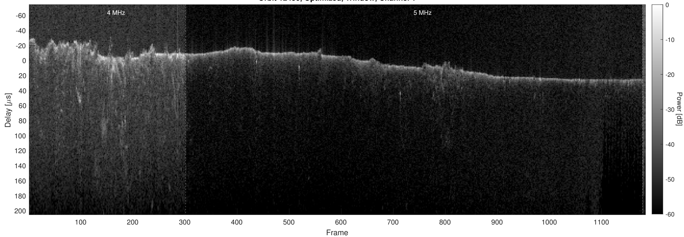
Orbit 12450, Optimized, Window, Channel 2
