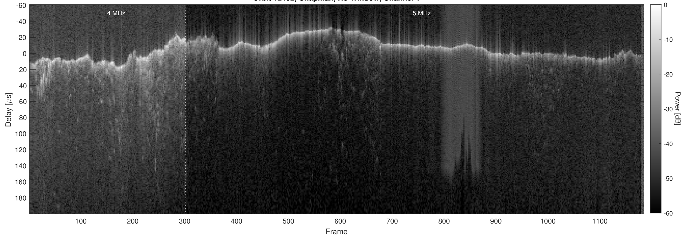
Orbit 12452, Chapman, No Window, Channel 2
