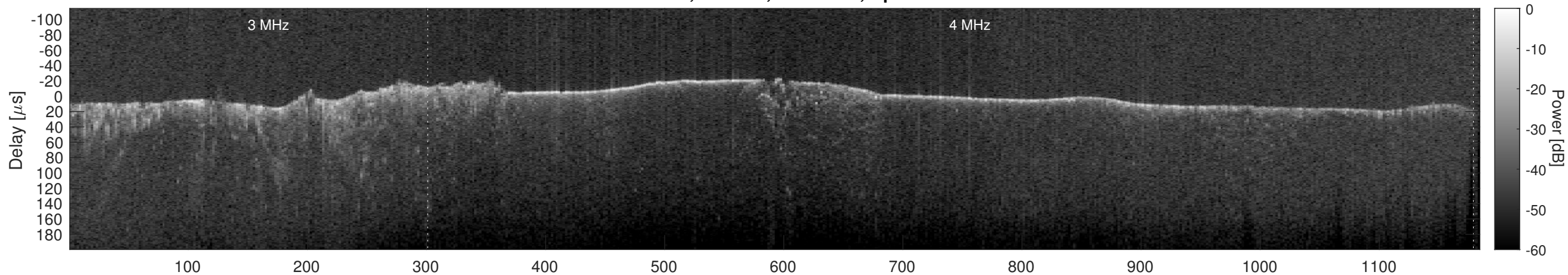
Orbit 12452, Cluttergram
