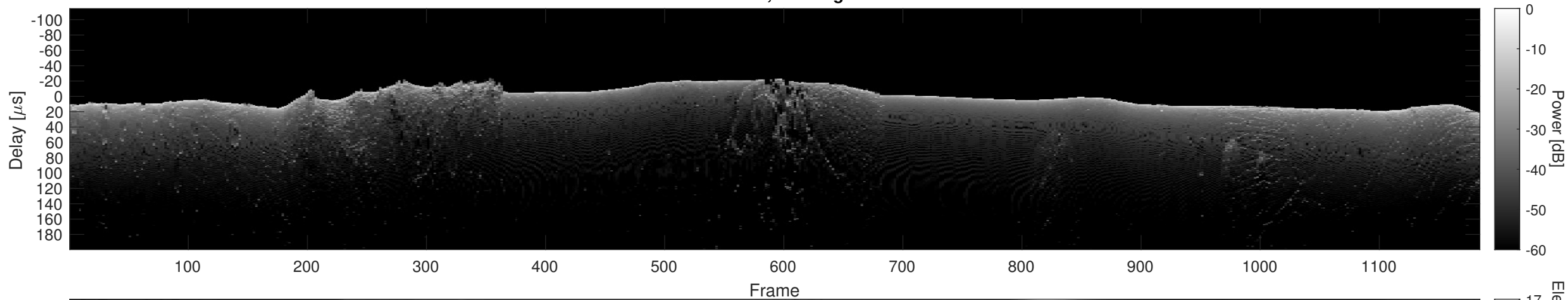
Orbit 12452, Cluttergram
