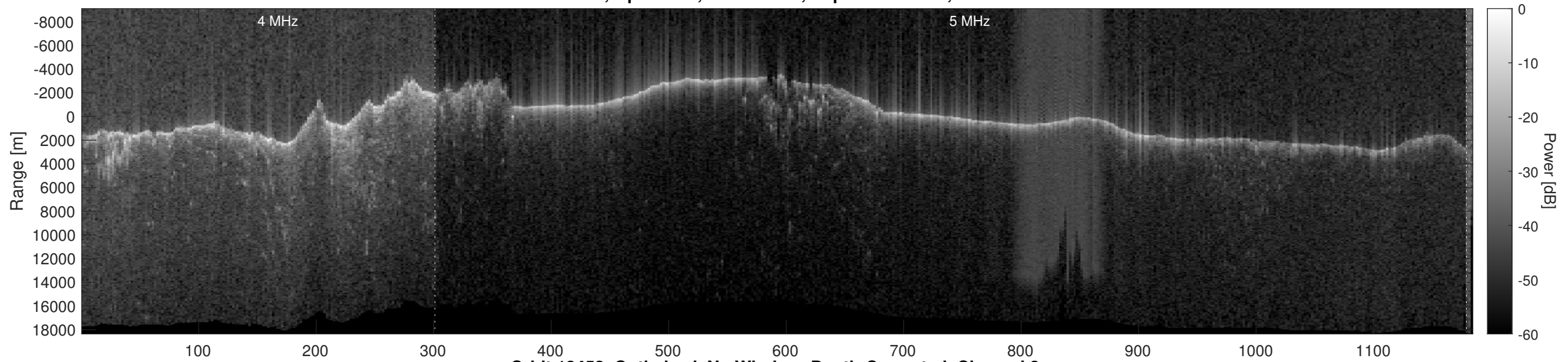
Orbit 12452, Optimized, No Window, Depth-Corrected, Channel 2
