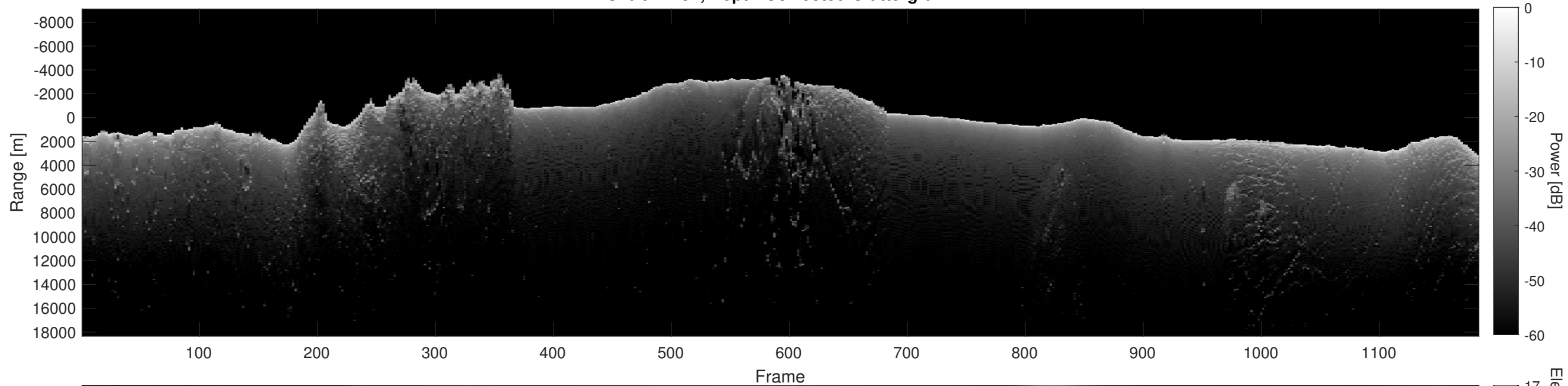
Orbit 12452, Depth-Corrected Cluttergram
