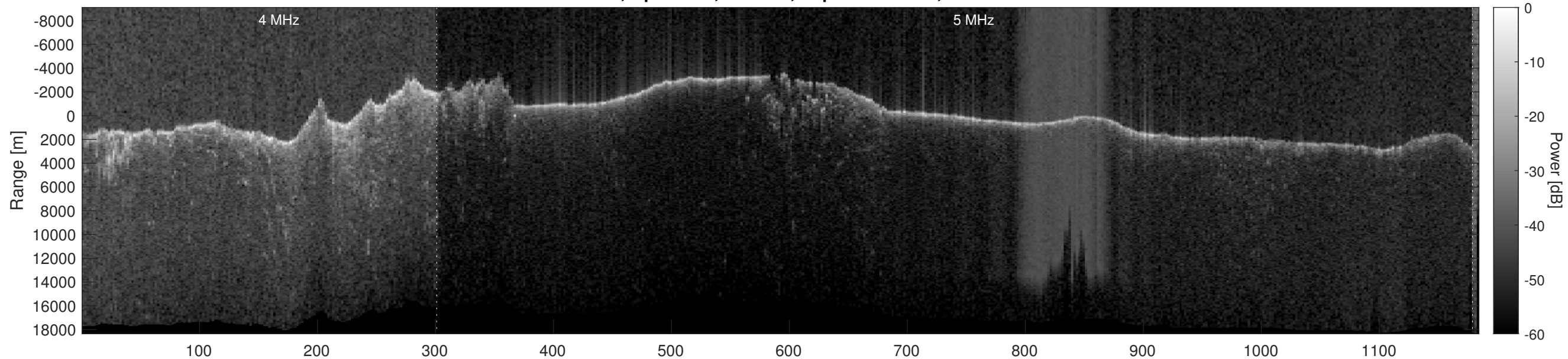
Orbit 12452, Optimized, Window, Depth-Corrected, Channel 2
