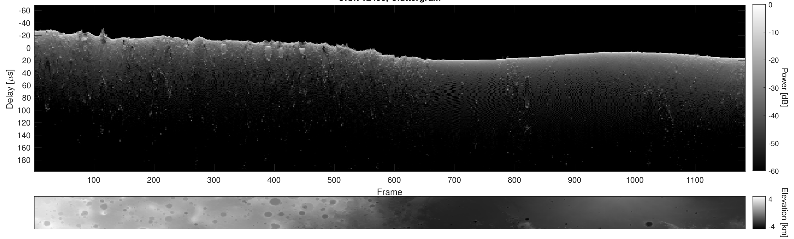
Orbit 12453, Cluttergram
