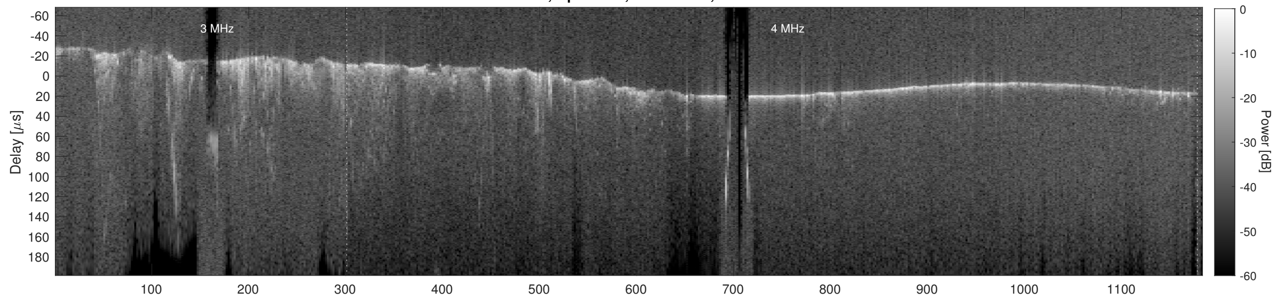
Orbit 12453, Cluttergram
