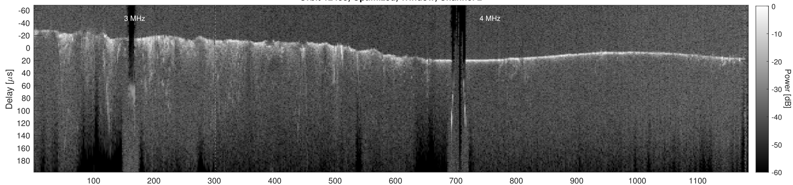
Orbit 12453, Cluttergram
