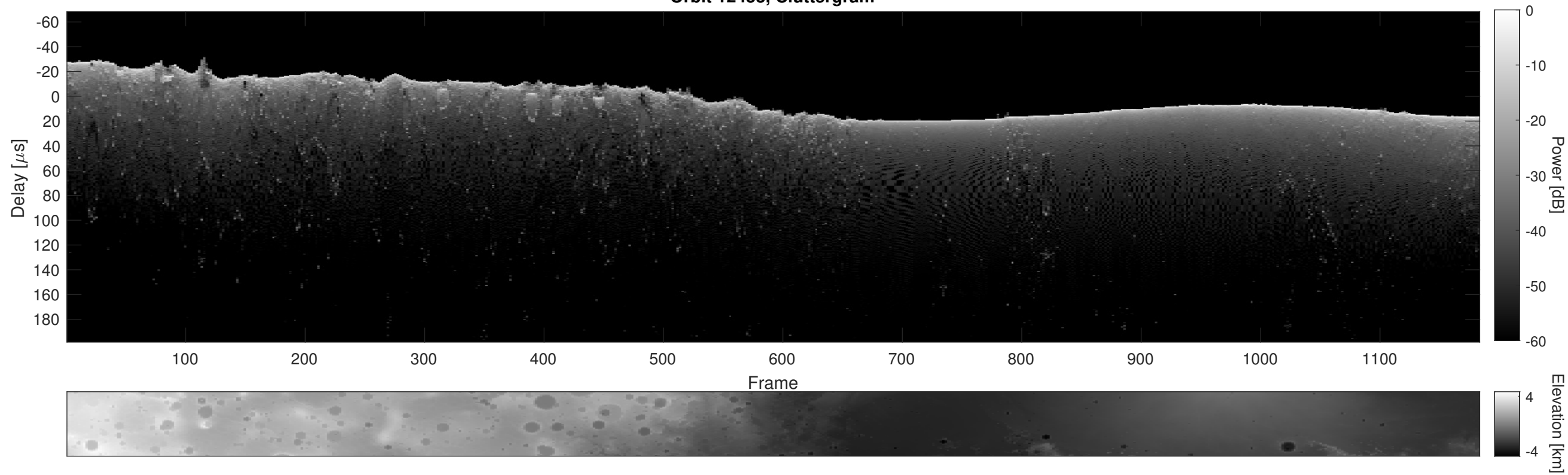
Orbit 12453, Cluttergram
