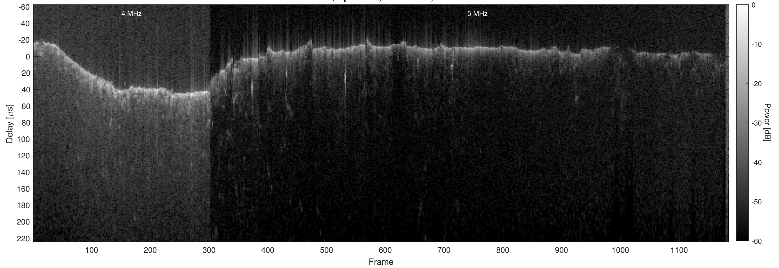
Orbit 12454, Optimized, No Window, Channel 2
