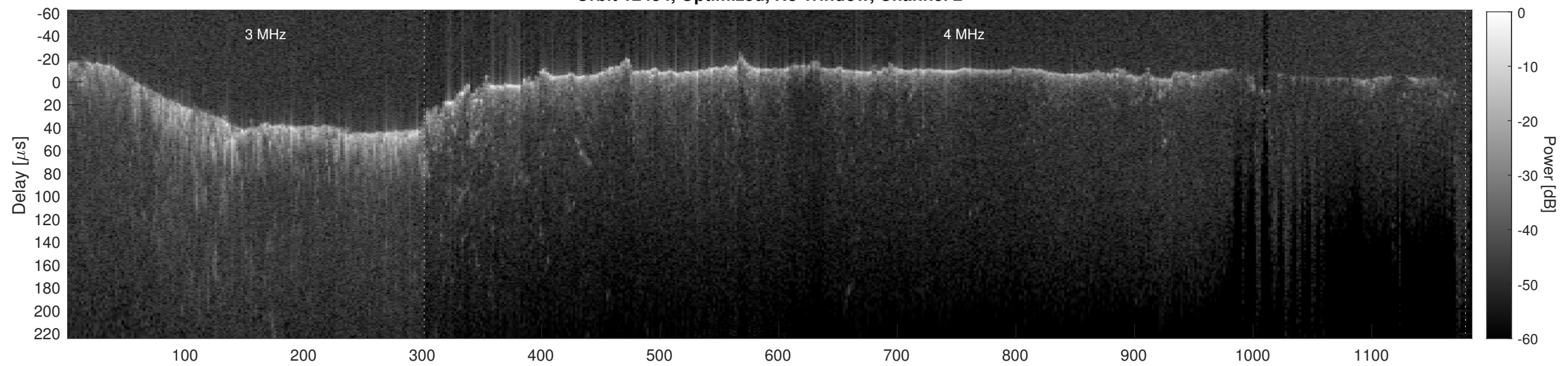
Orbit 12454, Cluttergram
