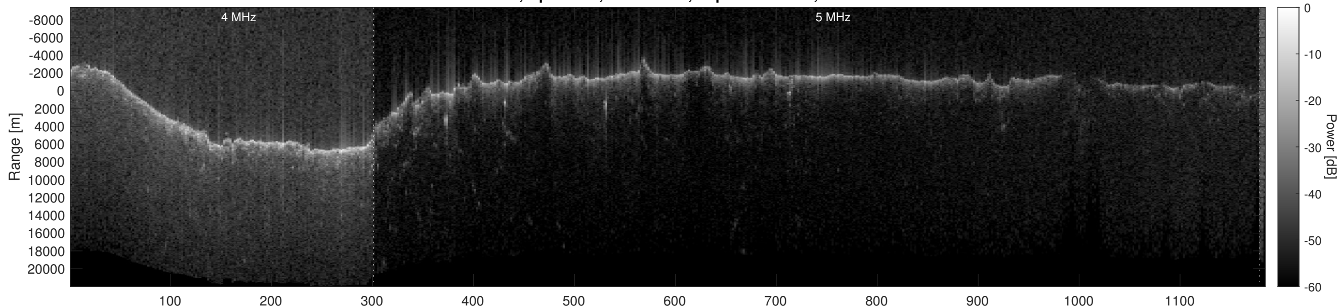
Orbit 12454, Optimized, No Window, Depth-Corrected, Channel 2
