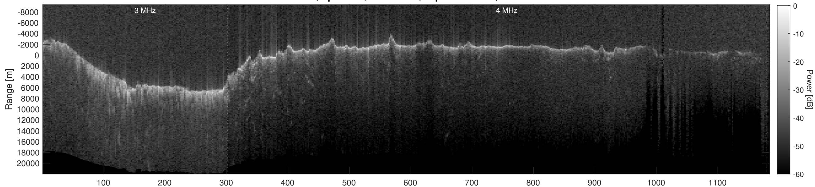
Orbit 12454, Depth-Corrected Cluttergram
