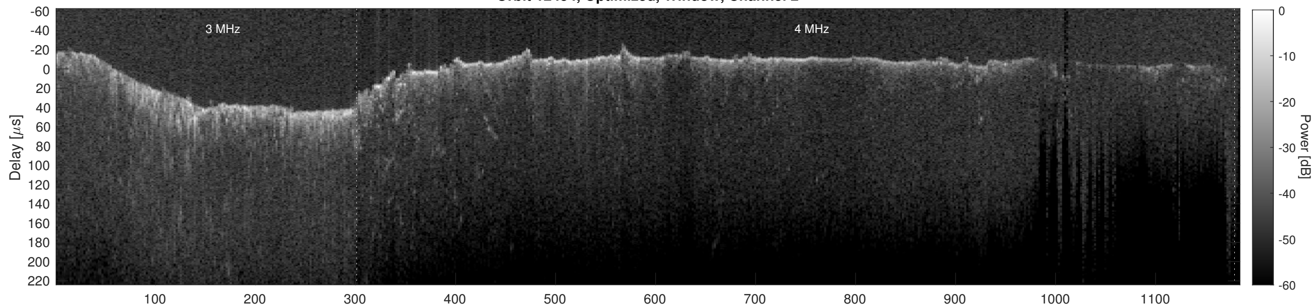
Orbit 12454, Cluttergram
