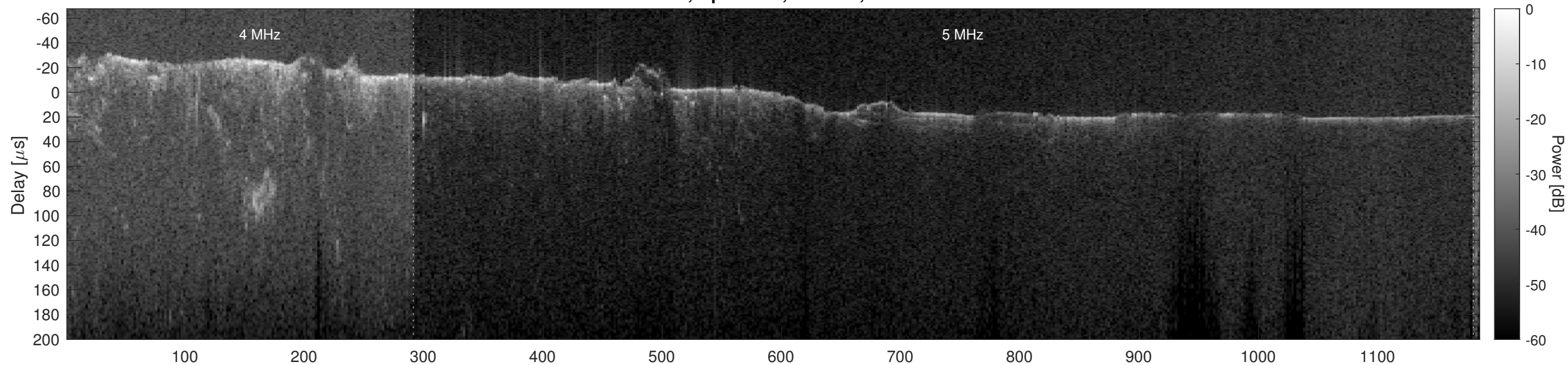
Orbit 12456, Optimized, Window, Channel 2
