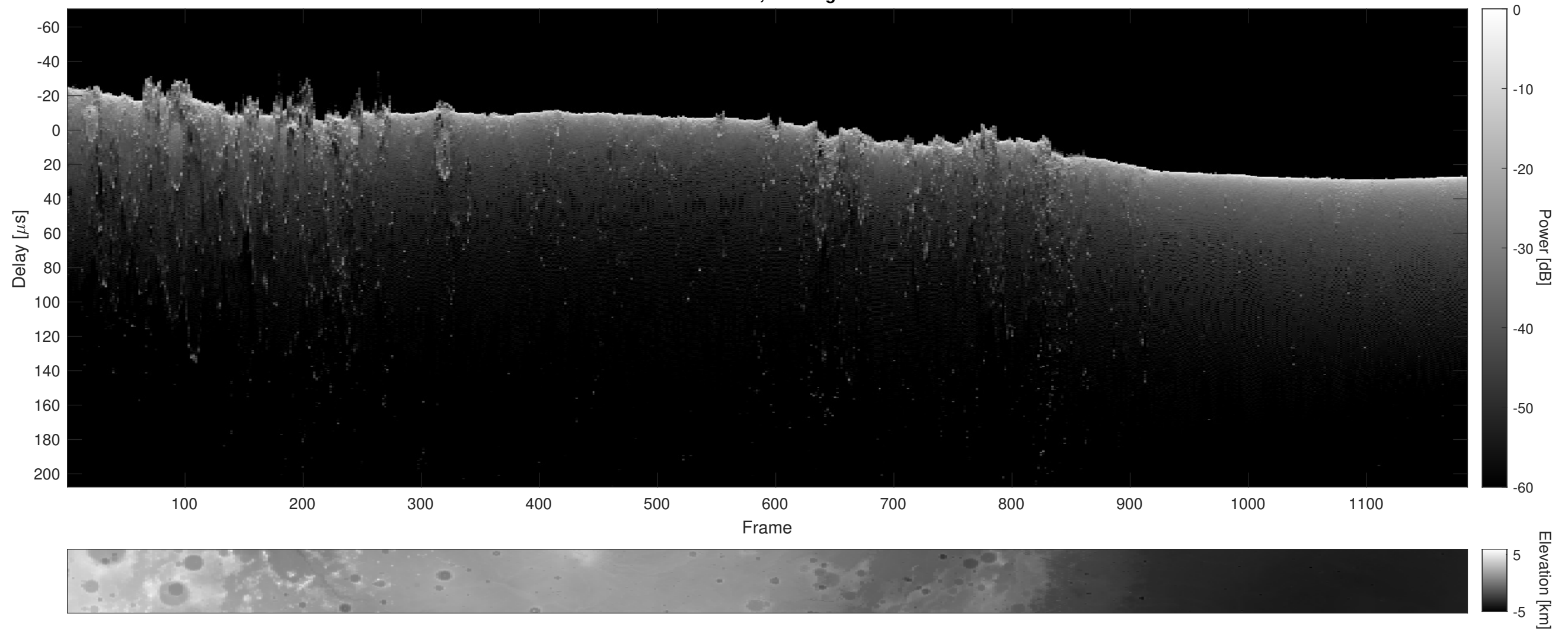
Orbit 12457, Cluttergram
