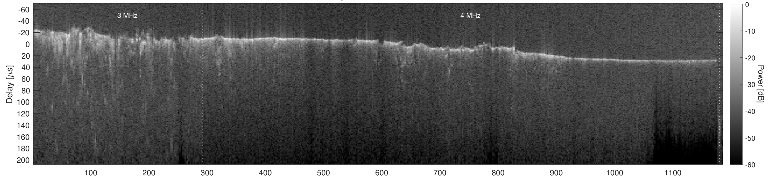
Orbit 12457, Cluttergram
