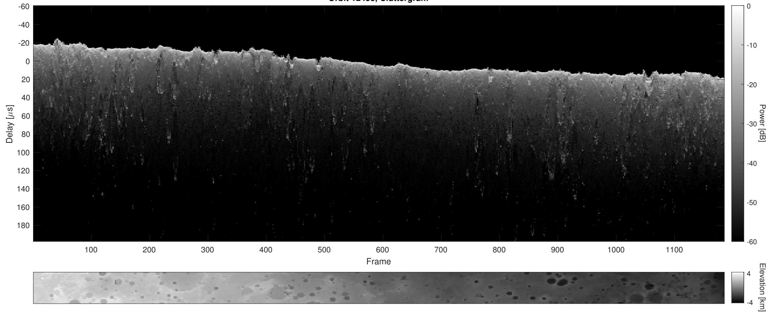
Orbit 12458, Cluttergram
