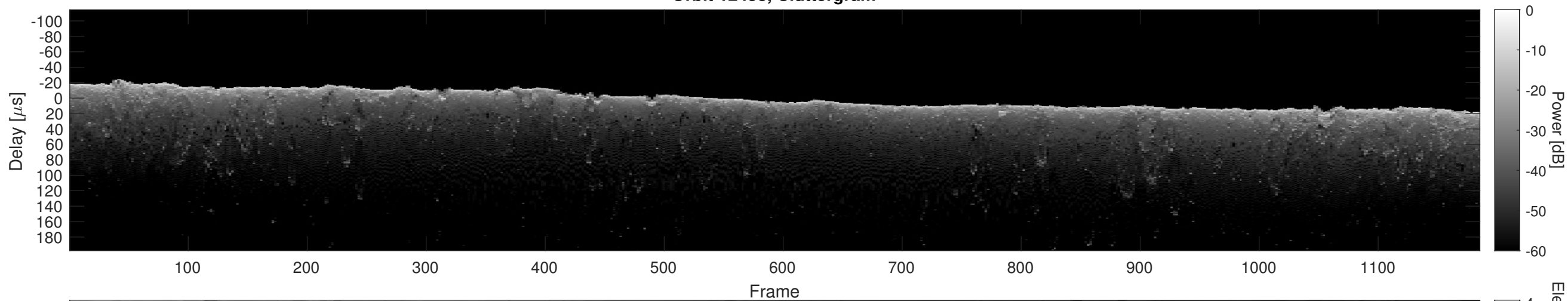
Orbit 12458, Cluttergram
