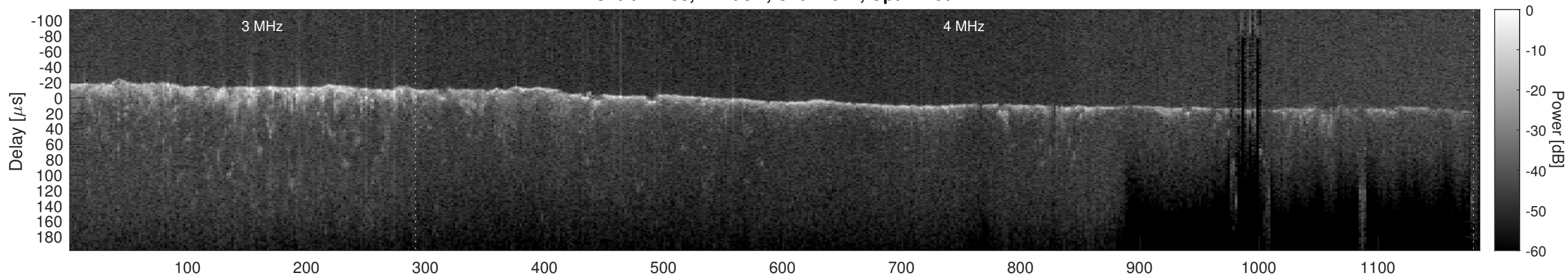
Orbit 12458, Cluttergram
