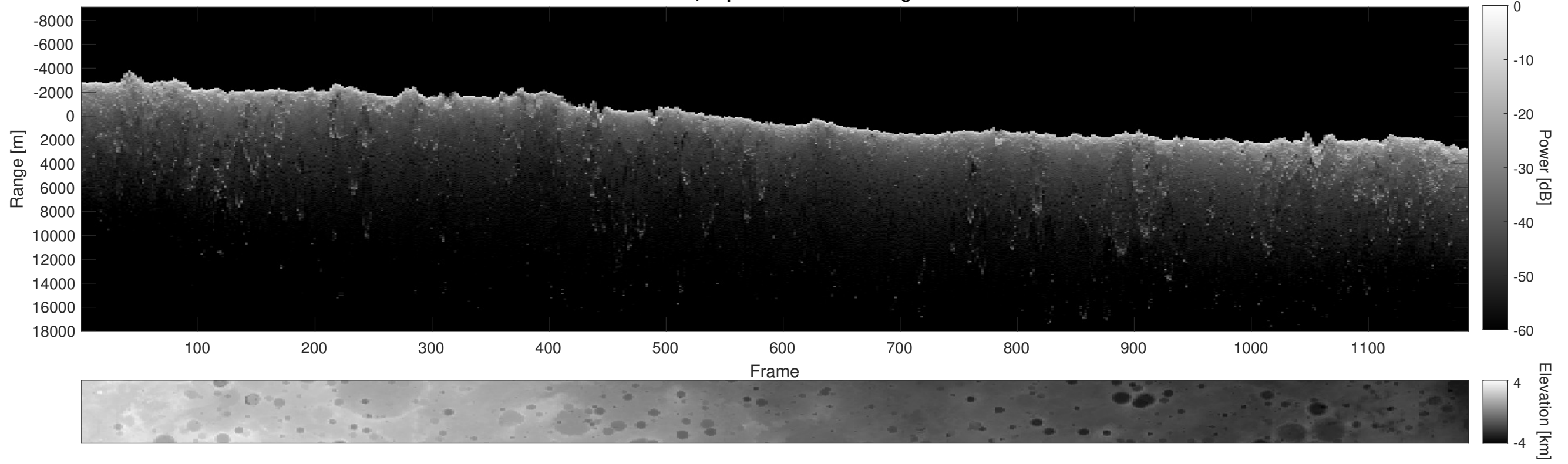
Orbit 12458, Depth-Corrected Cluttergram
