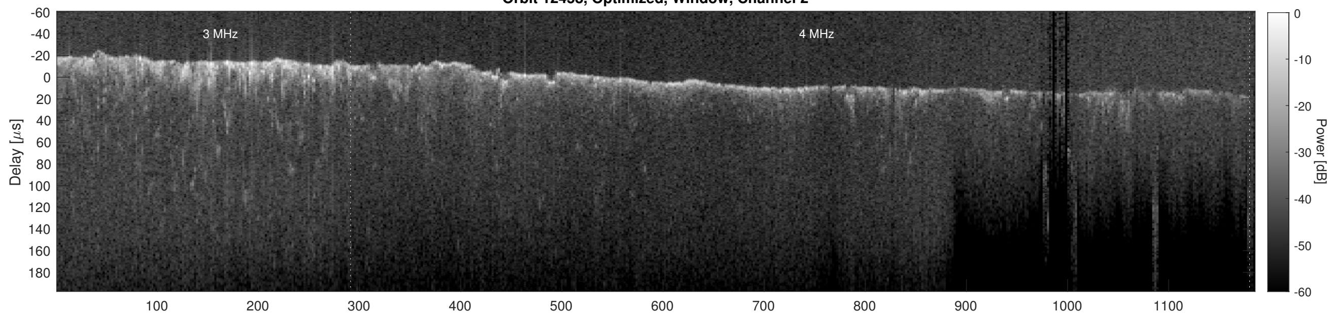
Orbit 12458, Cluttergram
