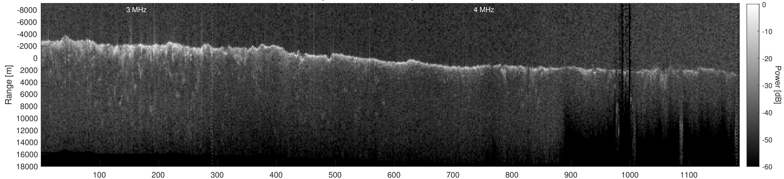
Orbit 12458, Depth-Corrected Cluttergram
