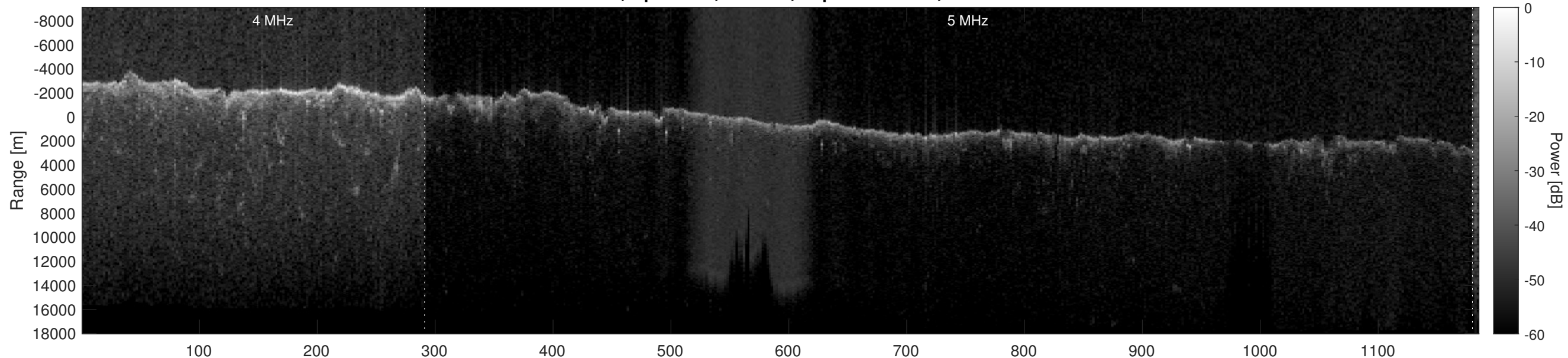
Orbit 12458, Optimized, Window, Depth-Corrected, Channel 2
