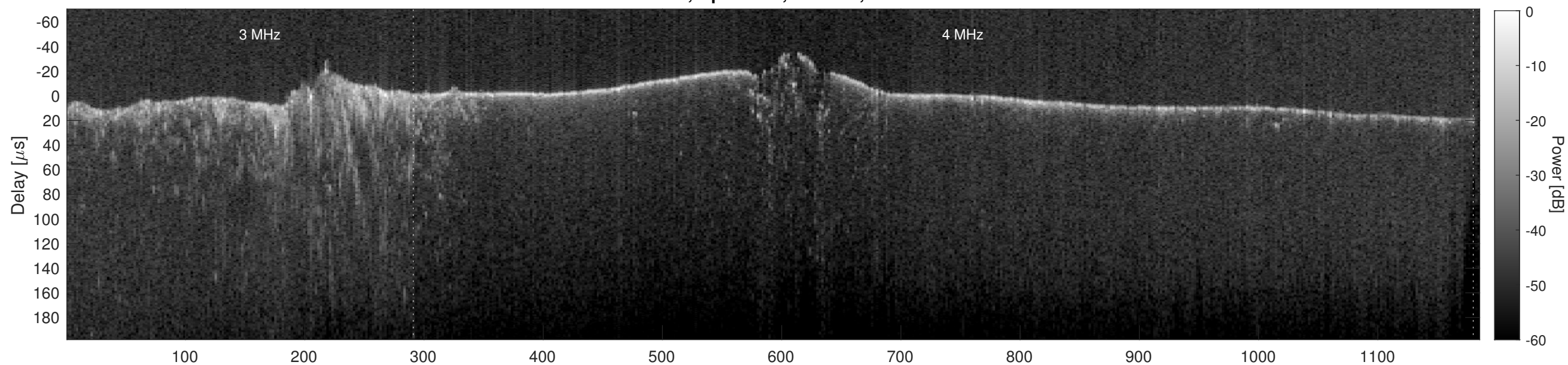
Orbit 12459, Cluttergram
