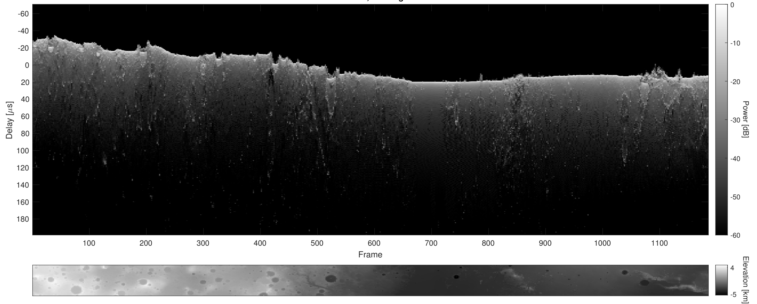
Orbit 12460, Cluttergram
