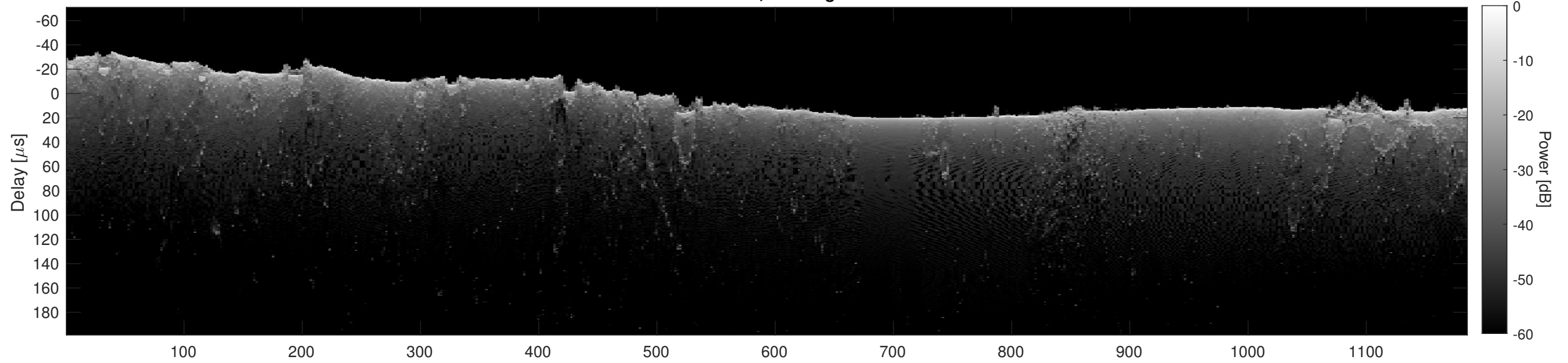
Orbit 12460, Cluttergram
