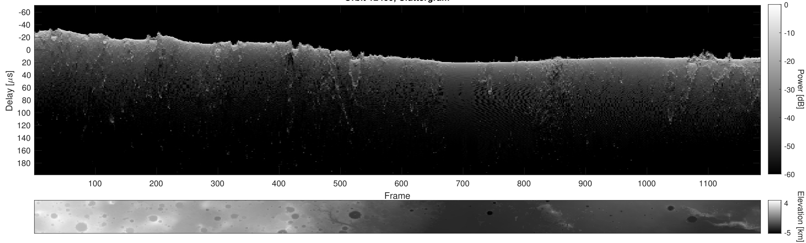
Orbit 12460, Cluttergram
