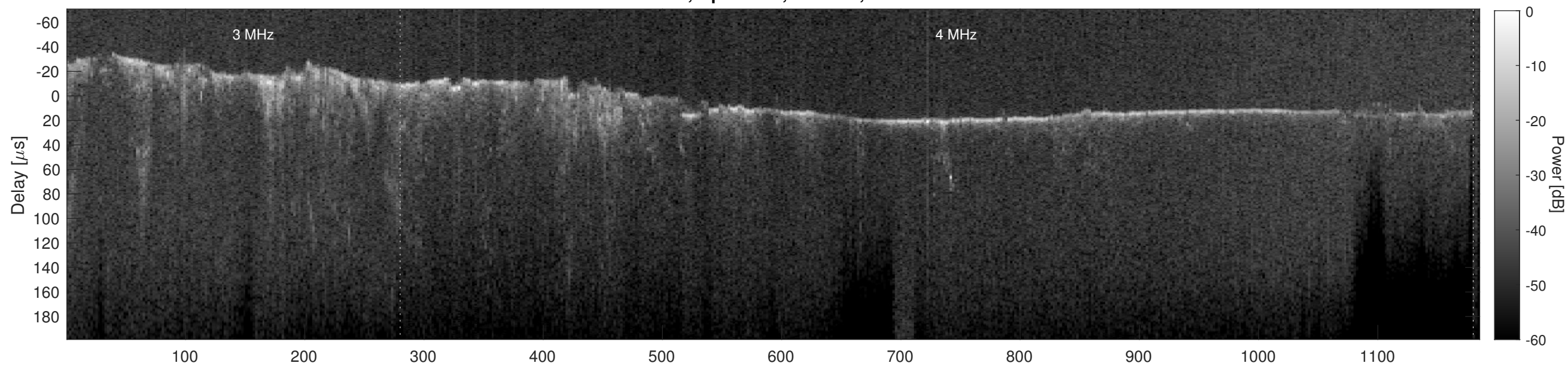
Orbit 12460, Cluttergram
