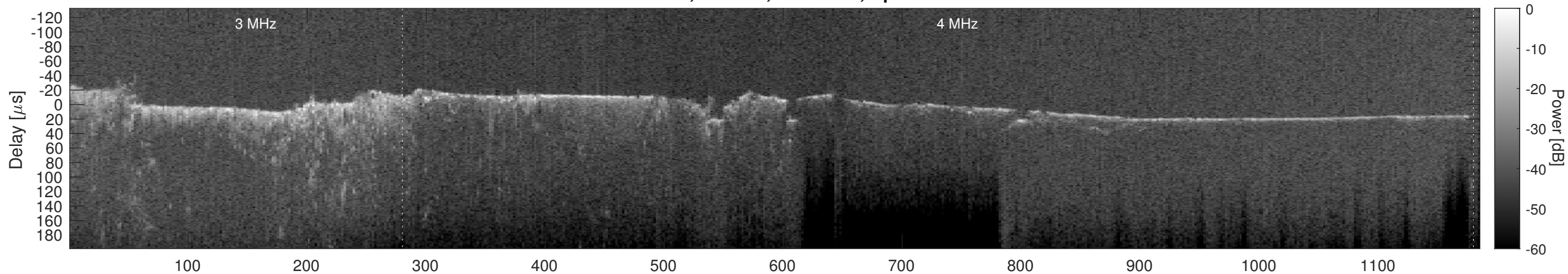
Orbit 12462, Cluttergram
