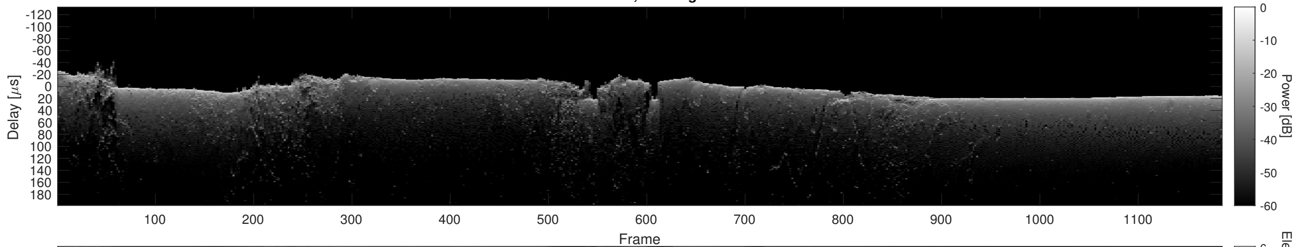
Orbit 12462, Cluttergram
