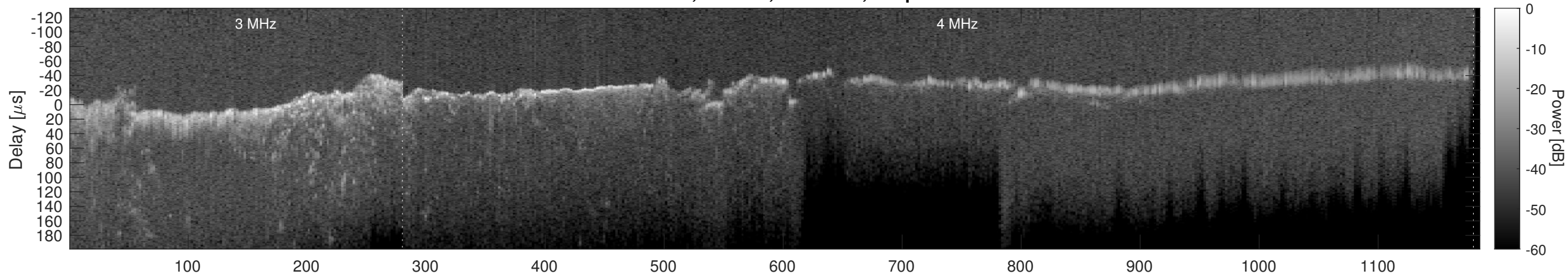
Orbit 12462, Window, Channel 2, Optimized
