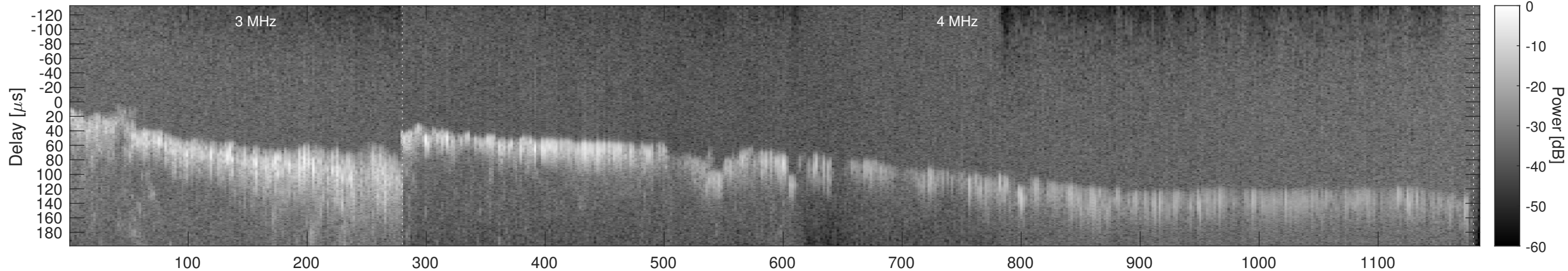
Orbit 12462, Window, Channel 2, Chapman
