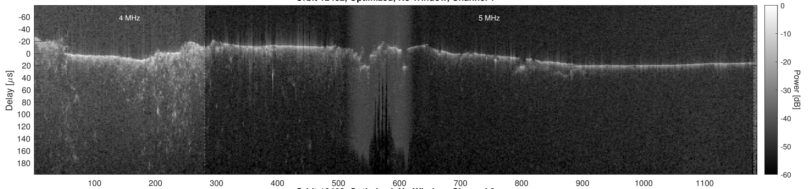
Orbit 12462, Optimized, No Window, Channel 2
