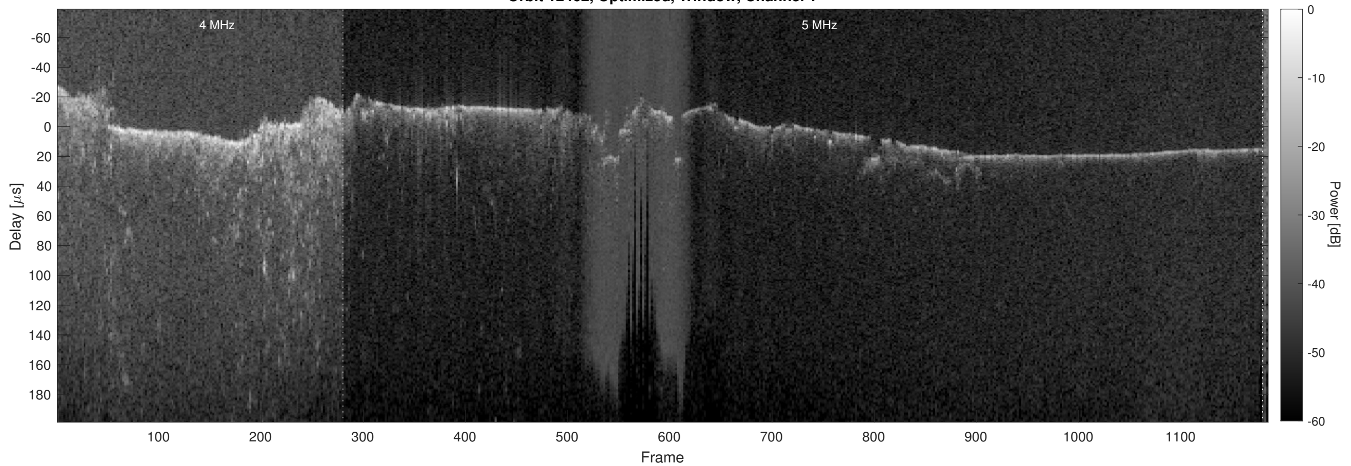
Orbit 12462, Optimized, Window, Channel 2
