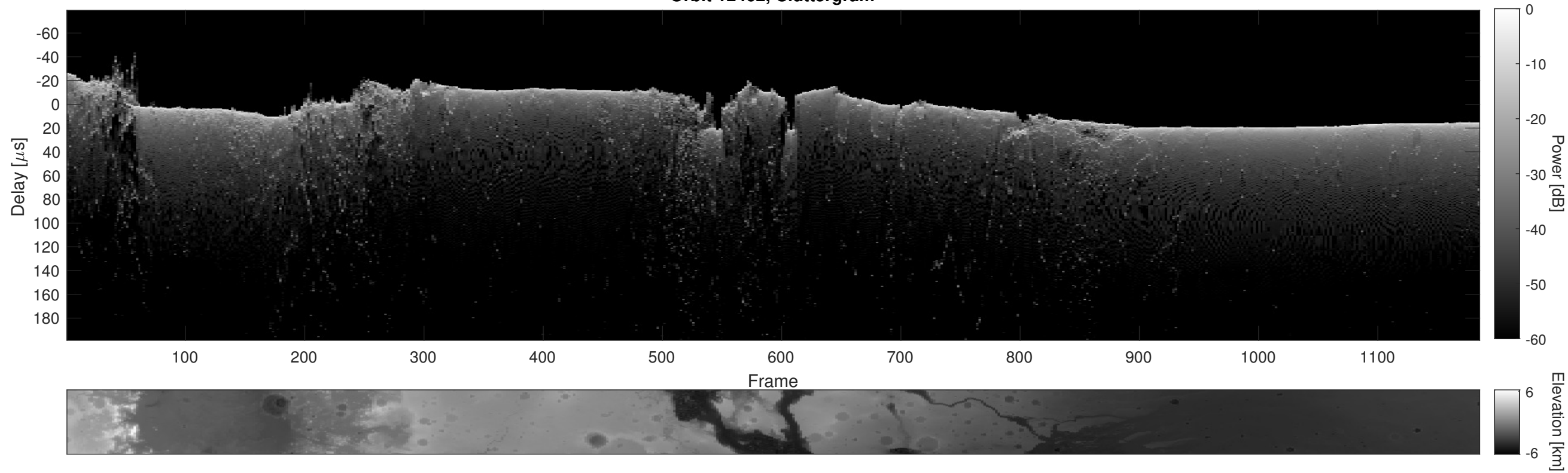
Orbit 12462, Cluttergram
