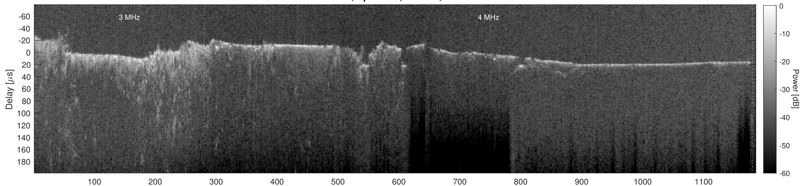
Orbit 12462, Cluttergram
