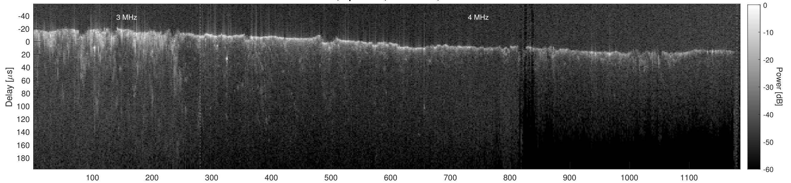
Orbit 12465, Cluttergram
