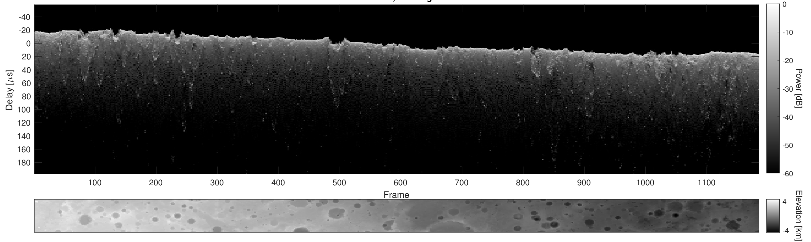
Orbit 12465, Cluttergram
