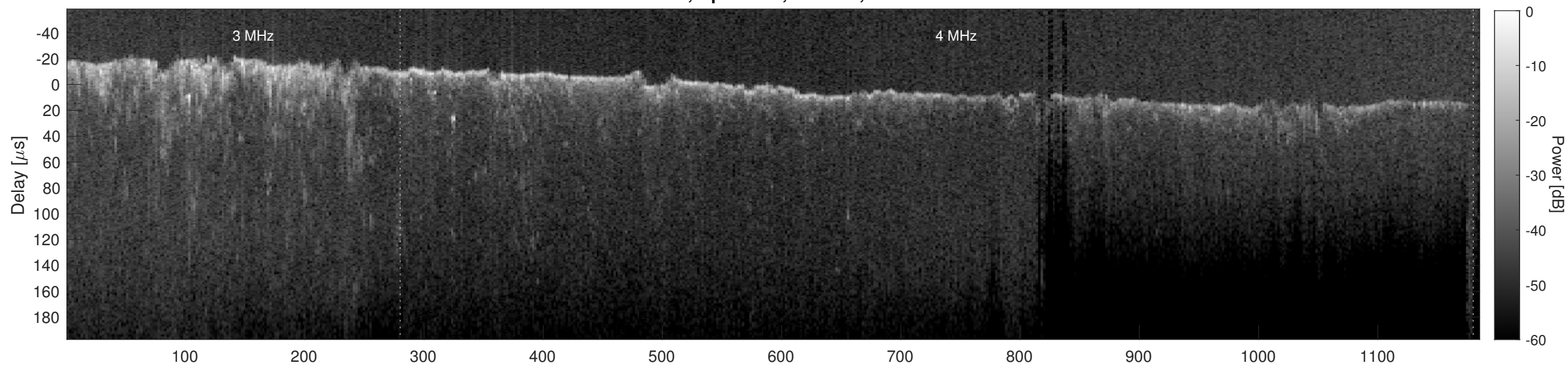
Orbit 12465, Cluttergram
