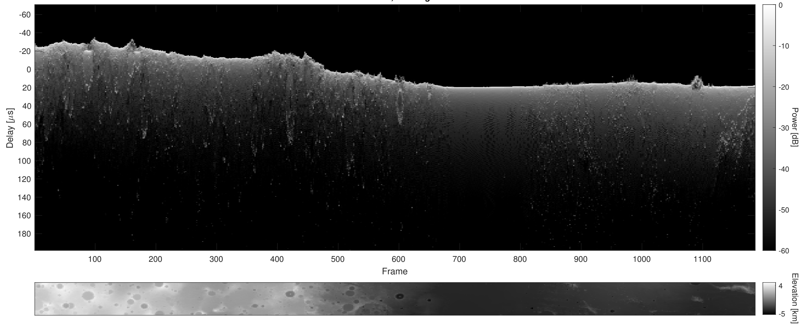
Orbit 12467, Cluttergram
