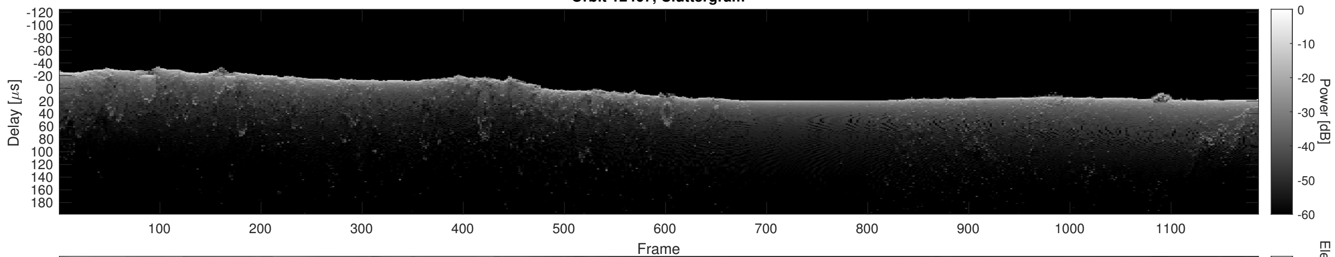
Orbit 12467, Cluttergram
