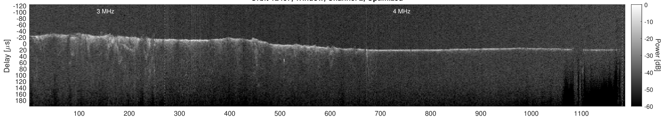
Orbit 12467, Cluttergram
