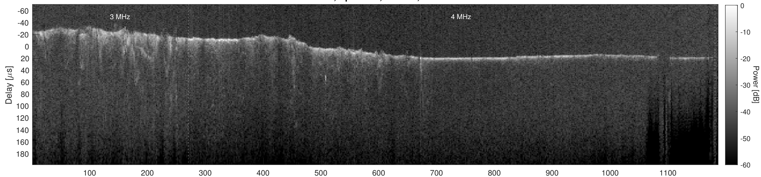
Orbit 12467, Cluttergram
