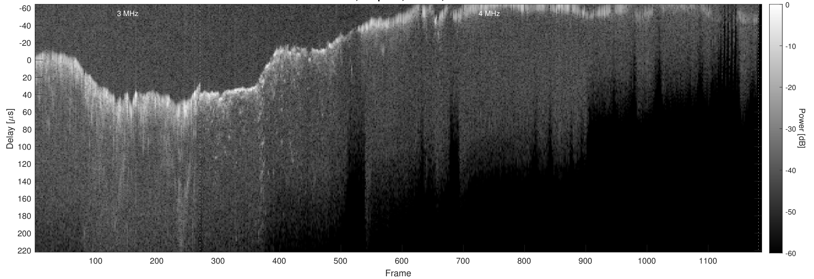
Orbit 12468, Chapman, Window, Channel 2
