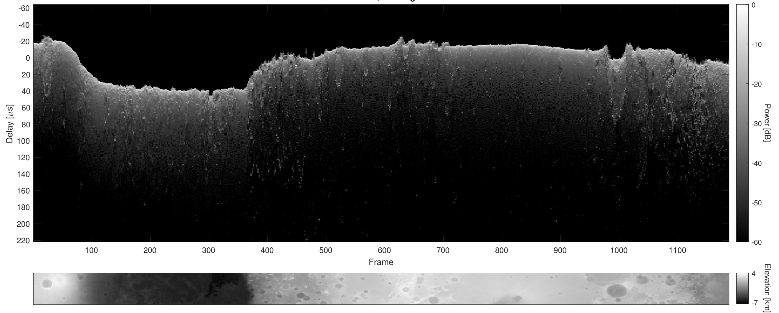
Orbit 12468, Cluttergram
