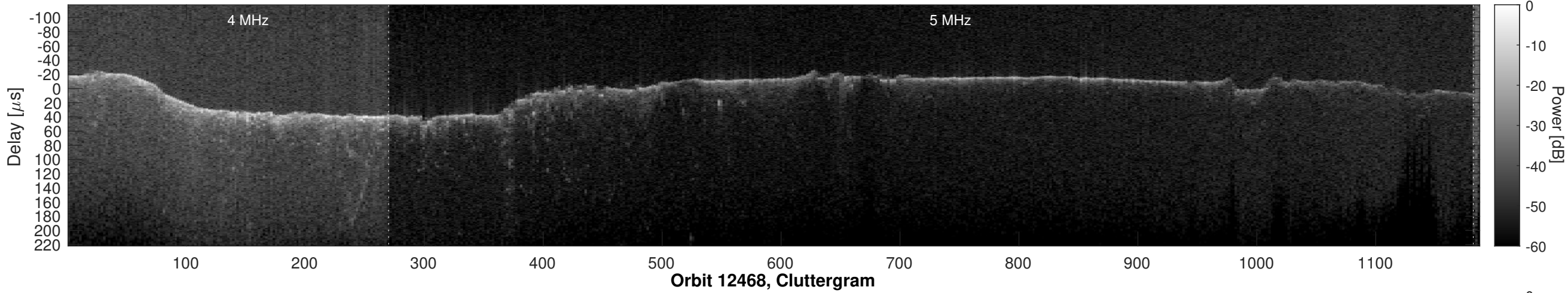
Orbit 12468, Window, Channel 1, Optimized
