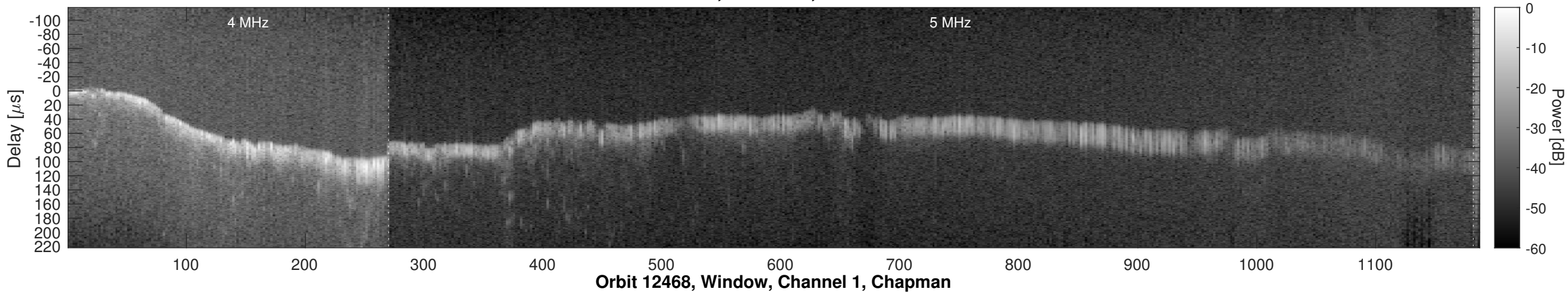
Orbit 12468, Channel 1, Uncorrected
